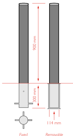
HC2065P Bollard (Powder Coat Finish)
